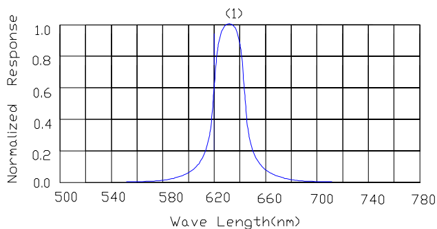
Spectral Reduance
