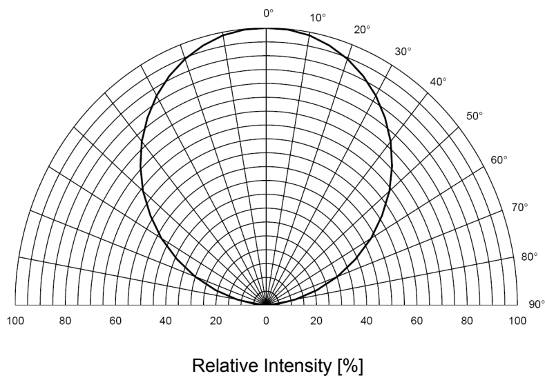
Radiation Characteristic T_a=25^\circ C
