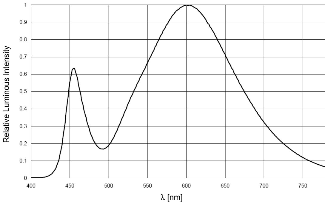
Relative Spectral Emission I_{v-rel} = f(\lambda); I_F=200mA, T_a=25^\circ C, T_J=30^\circ C
