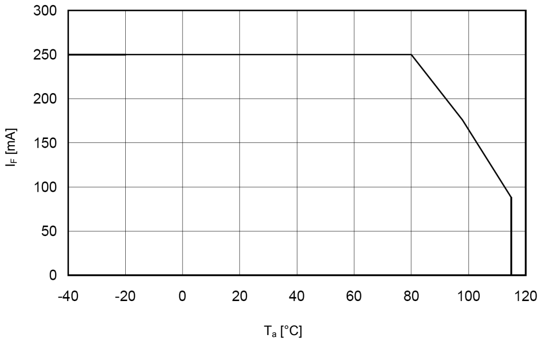
Allowable Forward Current vs Ambient Temperature
