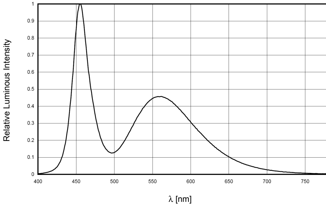
Relative Spectral Emission I_{v-rel} = f(\lambda); I_F=200\text{mA}, T_a=25^\circ\text{C}, T_J=30^\circ\text{C}
