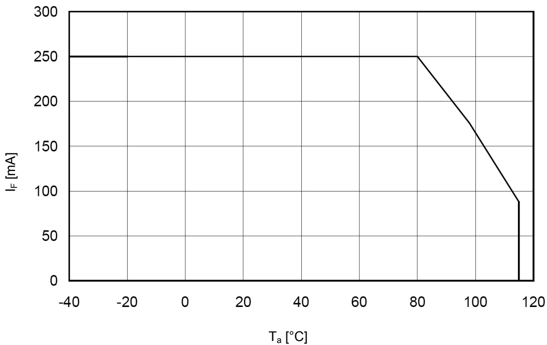
Allowable Forward Current vs Ambient Temperature
