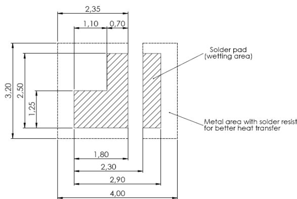
Recommended dimensions
