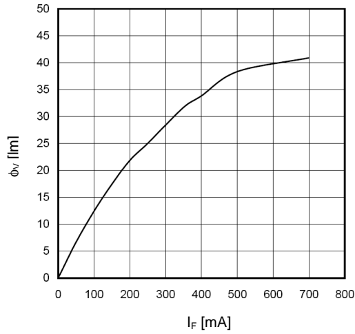
Luminous Flux \phi_V = f(I_F); T_A = 25\text{ °C}
