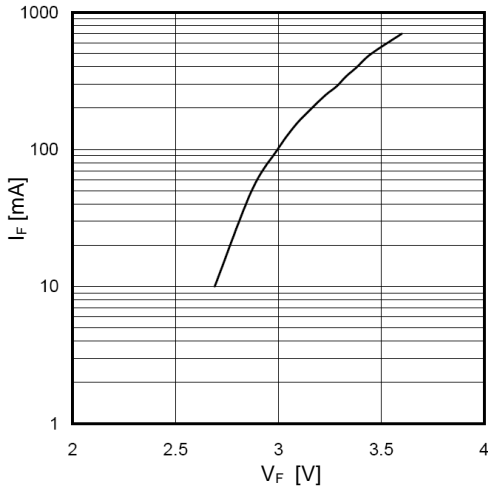
Forward Current I_F = f(V_F); T_A = 25\text{ °C}
