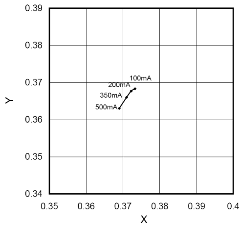
CIE-Shift XY = f(I_F); T_A = 25\text{ °C}
