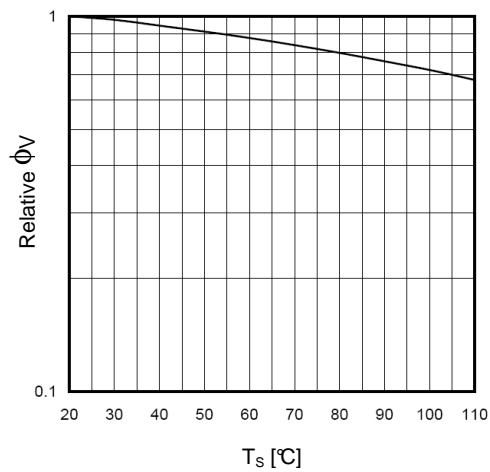
Luminous Flux \phi_{Vrel} = f(T_S); I_F = 350\text{ mA}
