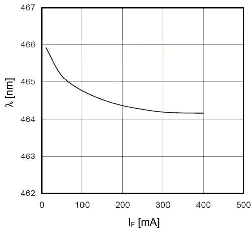
CIE-Shift \lambda = f(I_F); T_A = 25\text{ °C}
