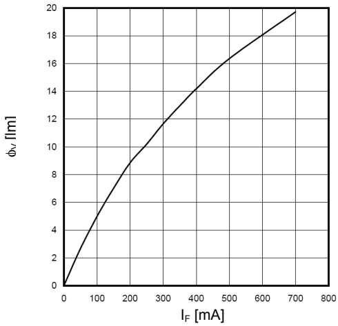
Luminous Flux \phi_V = f(I_F); T_A = 25\text{ °C}
