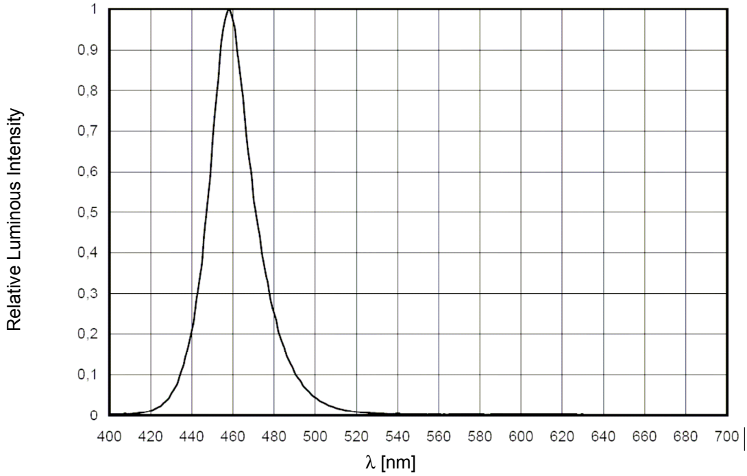
Relative Spectral Emission I_{v-rel} = f(\lambda); I_F=350mA, T_a=25^\circ C
