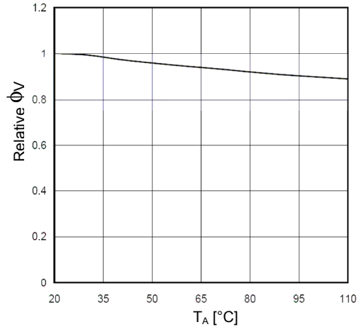
Luminous Flux \phi_{Vrel} = f(T_A); I_F = 350\text{ mA}
