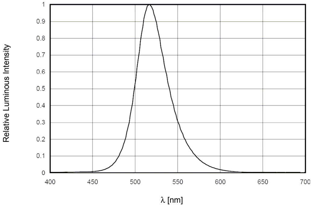
Relative Spectral Emission *) I_{v-rel} = f(\lambda); I_F=200mA, T_a=25^\circ C
