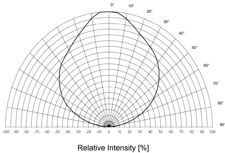
Radiation Characteristic T_a=25^\circ C
