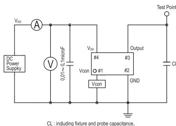
CL : including fixture and probe capacitance.
