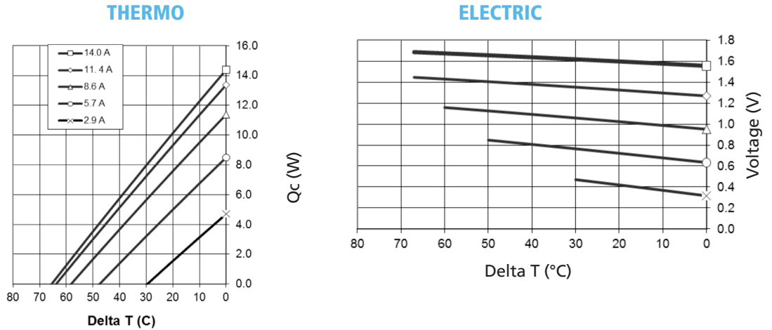
Performance Curves at Th = 25°C
