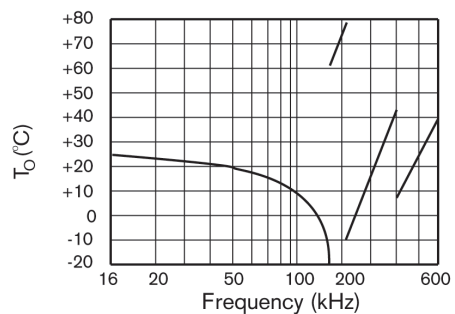
FIGURE 4 CX2V TYPICAL TURNING POINT TEMP. ( T_0 )
