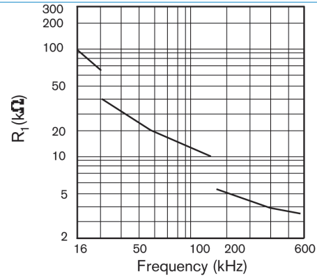
FIGURE 2 CX2V TYPICAL MOTIONAL CAPACITANCE ( C_1 )
