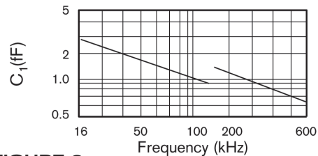
FIGURE 3 CX2V TYPICAL QUALITY FACTOR ( Q )
