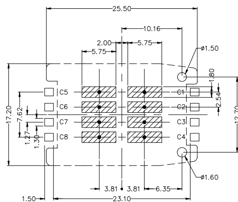
Unit: mm; Tolerances: ±0.10mm Mechanical outline dimension
