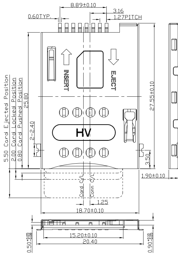
Unit: mm; Tolerances: ±0.15 mm Mechanical outline dimension
