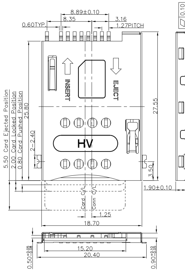
Unit: mm; Tolerances: ±0.15 mm Mechanical outline dimension
