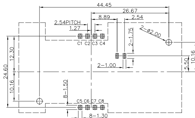
Unit: mm, Tolerances: ±0.05 mm Reference dimension for PCB layout
