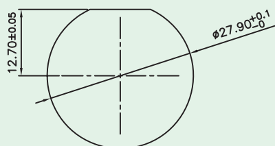
Panel Cut-Out Panel Thick: 1.5~3.2mm
