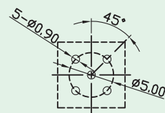
PCB Cut-out
