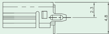
PCB LAYOUT/TOP VIEW
