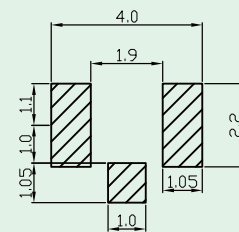
PCB LAYOUT
