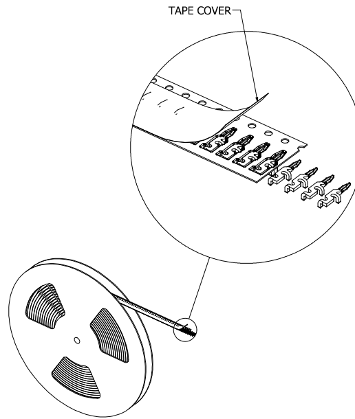
IPX15277-03 ON TAPE & REEL 13" DIA PLASTIC REEL 5,000 PARTS PER REEL
