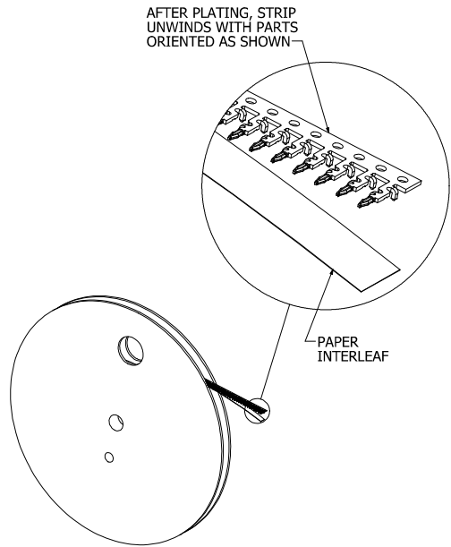
IPX15277-01 ON REEL W/ CARRIER 15" DIA CORRUGATED PLASTIC REEL 5,000 PARTS PER REEL
