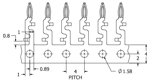
DETAILS OF IPX15277-01 ON REEL W/ CARRIER
