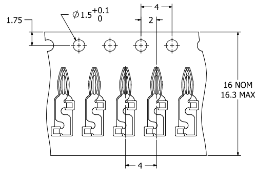
DETAILS OF IPX15277-03 ON TAPE & REEL
