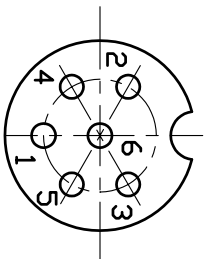
Arrangement of Contact
