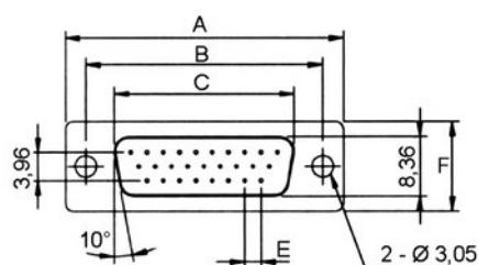
Stift / Male
