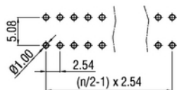
Single Slot
