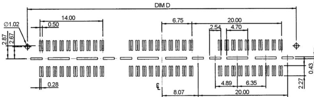
Recommended PCB Layout Tolerances \pm 0.03
