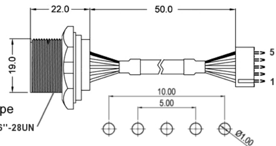
Flying Lead PCB Layout
