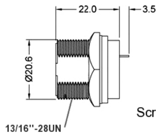
13/16''-28UN
