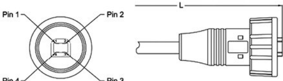
Waterproof USB B Male Straight ...-2-1-XX
