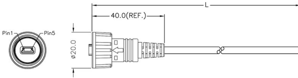
Waterproof Mini-USB B Male Straight WA826-3-1-37-...
