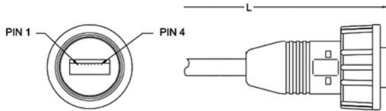
Waterproof USB A Male Straight ...-1-1-XX
