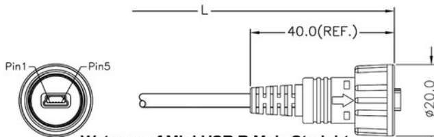
Waterproof Mini-USB B Male Straight ...-3-1-37
