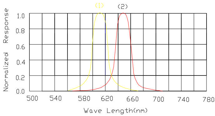
Spectral Reduance
