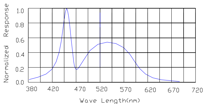
Spectral Radiance
