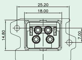
PANEL SIDE
