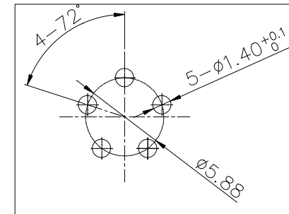
Pin Layout PCB
