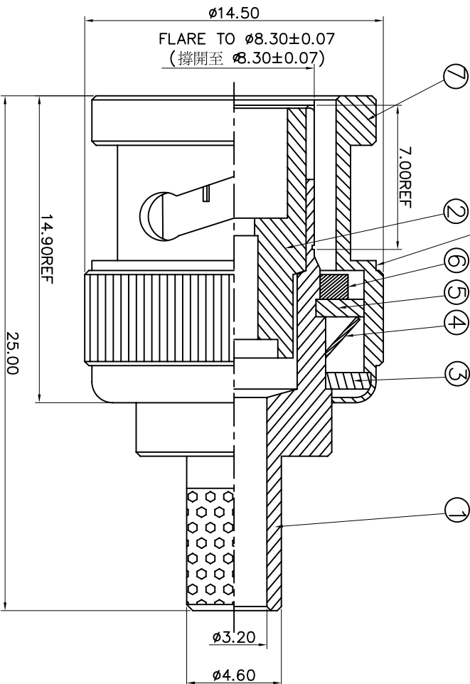
STAKE IN 3 PLACES EQUALLY SPACED 120° APART (打三點，間隔120°)
