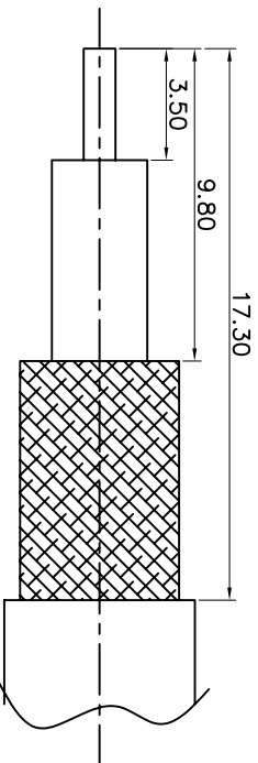
FE COMMENDED CABLE STRIPPING DIM'S (建議剖線尺寸)
