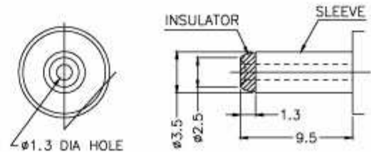
Fig. 8 MATCHING PLUG
