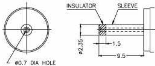
Fig. 3 MATCHING PLUG
