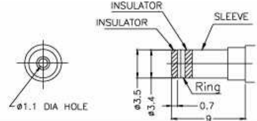
Fig. 6 MATCHING PLUG
