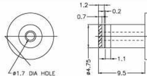
Fig. 9 MATCHING PLUG
