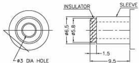
Fig. 10 MATCHING PLUG
