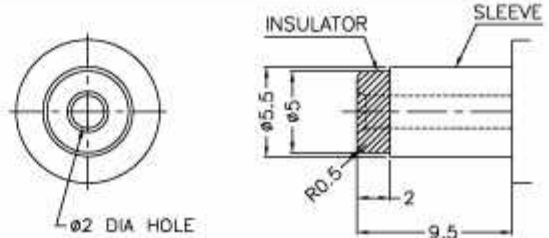
Fig. 10 MATCHING PLUG
