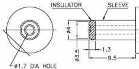
Fig. 7 MATCHING PLUG
