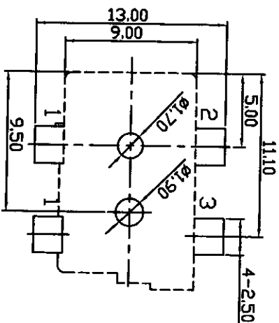
Pin Hole Layout (Jack Bottom View)
