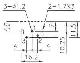
Pin Hole Layout (Jack Bottom View)
