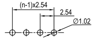
PCB Layout
